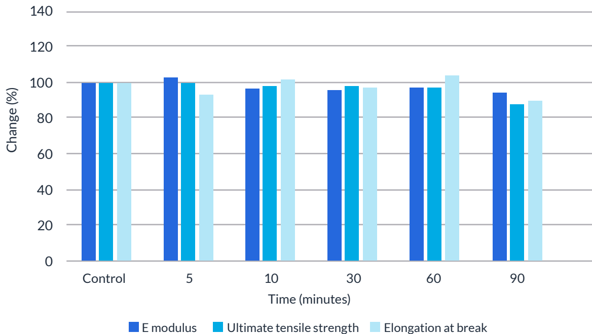
Change in mechanical properties, 75°C
